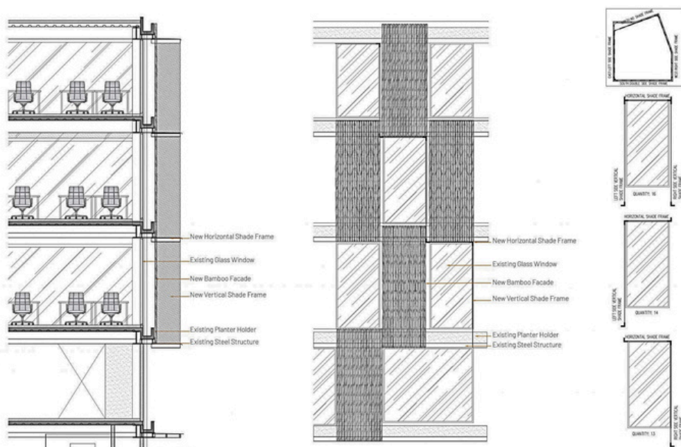
Wall to Facade Detail
